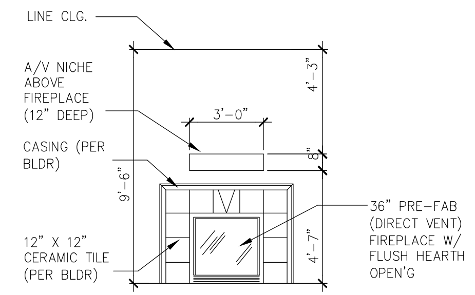
NICHE DETAIL UNIT #41 SCALE: 1/4" = 1'-0"
